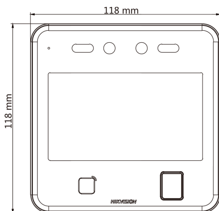
Dimension with Fingerprint Module
