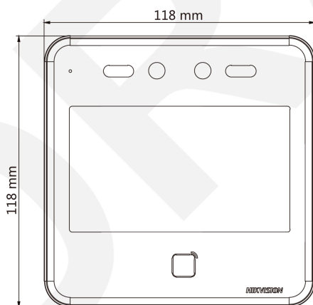
Dimension without Fingerprint Module
